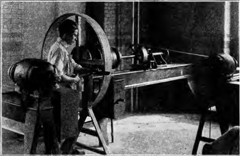
FIG. 407. WORKING SEGMENTAL CORE TO SHAPE.
